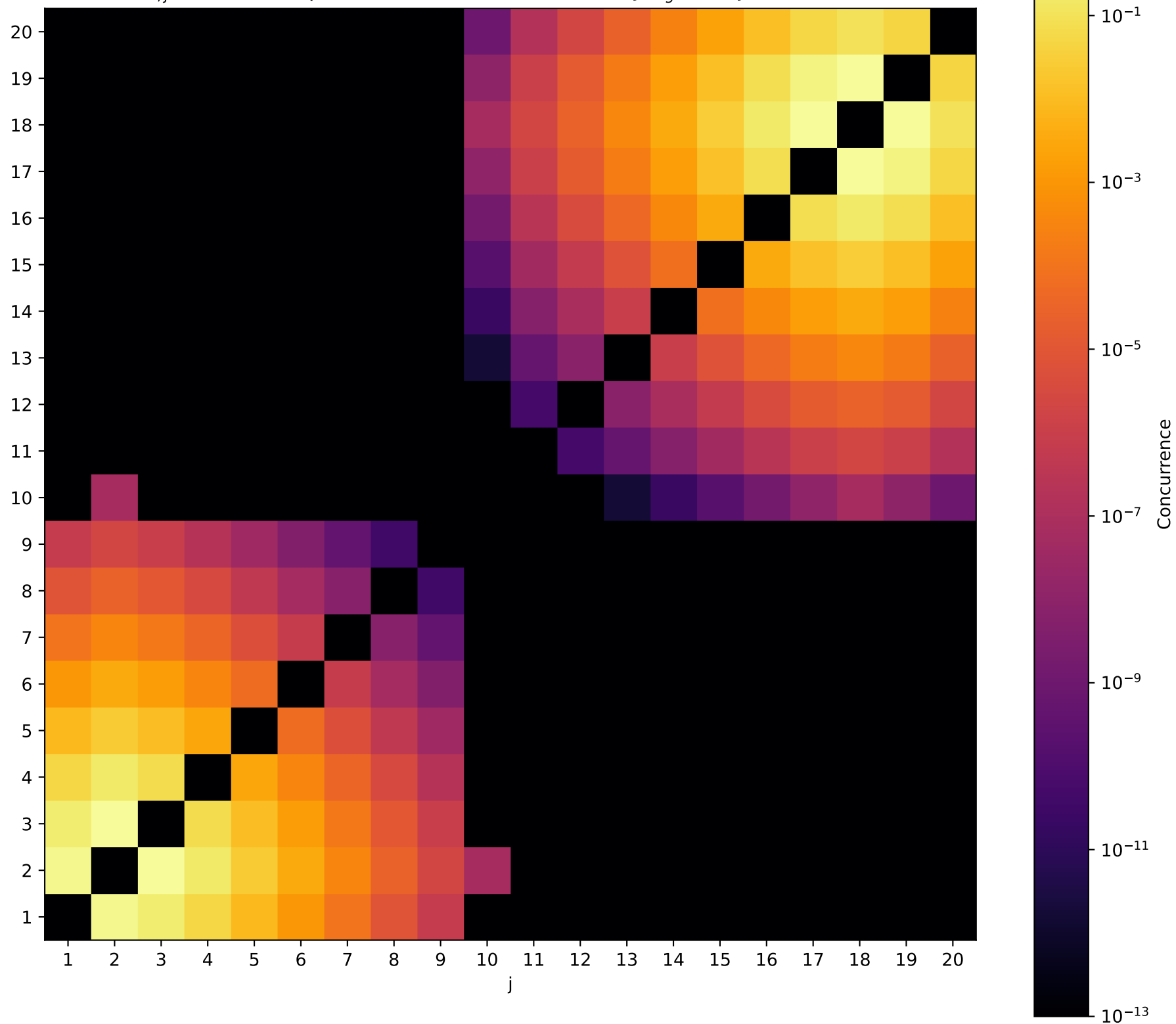
C_{i,j}(t = 0.50) for product state (2,18) (band 2) - J_{long} = 20, J_z = 1, \alpha = 0.5
